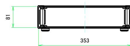
B-B (1:6)
