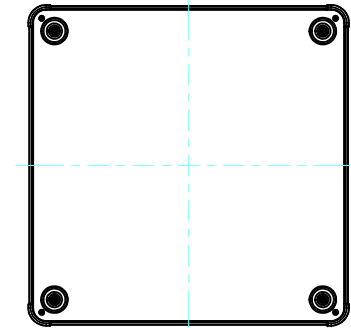
C-C (1:6)
